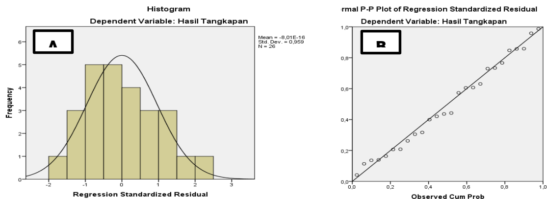
Gambar 3. Grafik Histogram (A) dan Normal P-P plot of Regression Standardized Residual (B)
