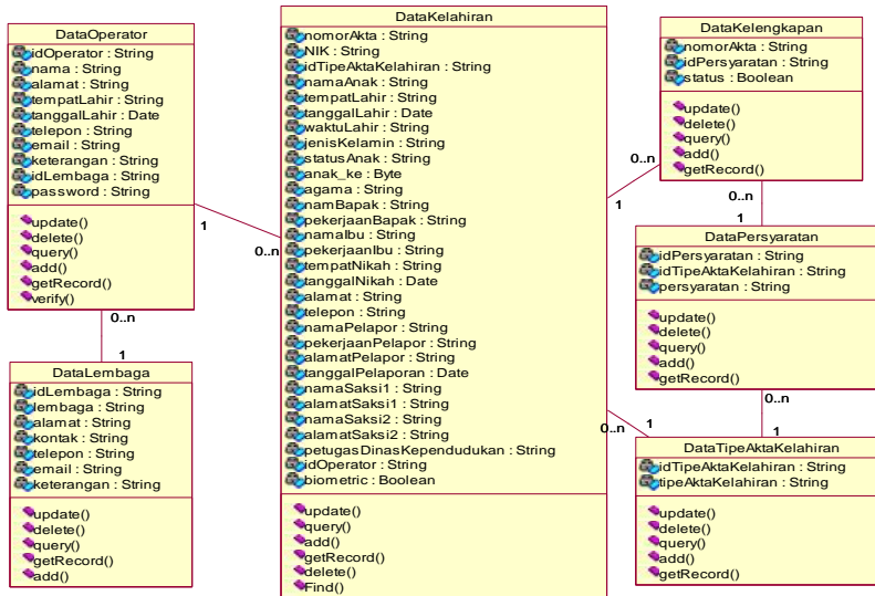
Class Diagram
