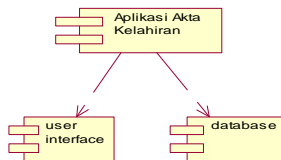
Component Diagram
