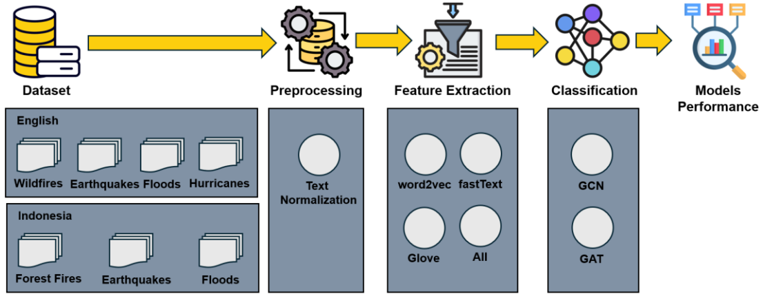
Figure 1. Research flow.
