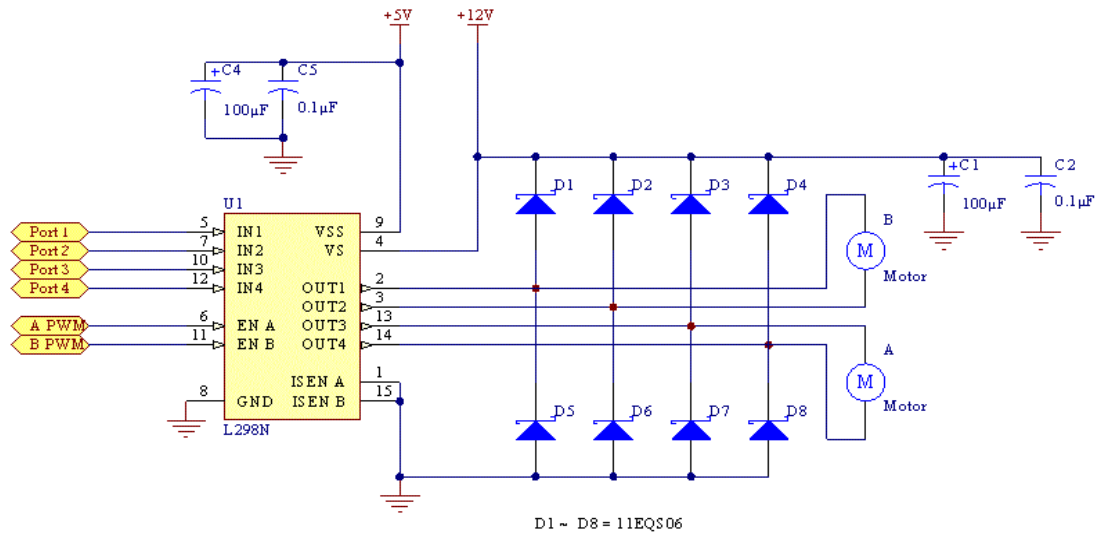
Figure 4. Schematic IC L298N as DC motor driver [5]
