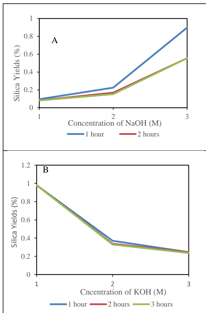
Figure 3. Effect of extraction time on the extraction yield of CFA B silica with NaOH (A) and KOH (B) solvents.
