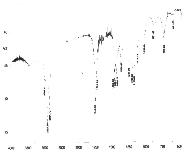
Gambar 2. Spektra FT-IR biodiesel
