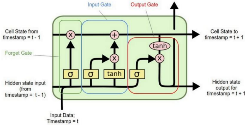
Figure 3. LSTM Architectures
