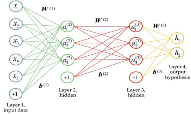
Figure 2. Neural Network Architectures
