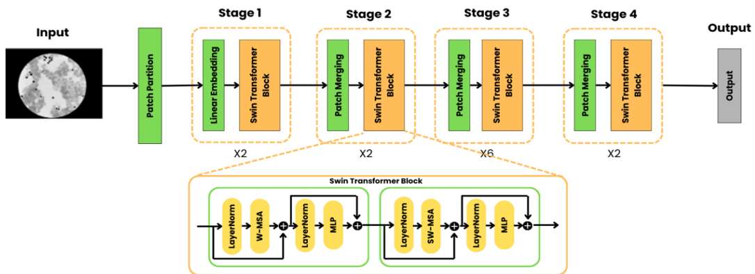
Figure 4. Swin Transformer Architecture
