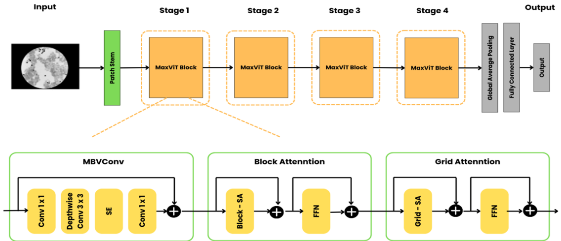
Figure 6. MaxViT Architecture
