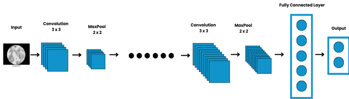
Figure 1. CNN Architecture
