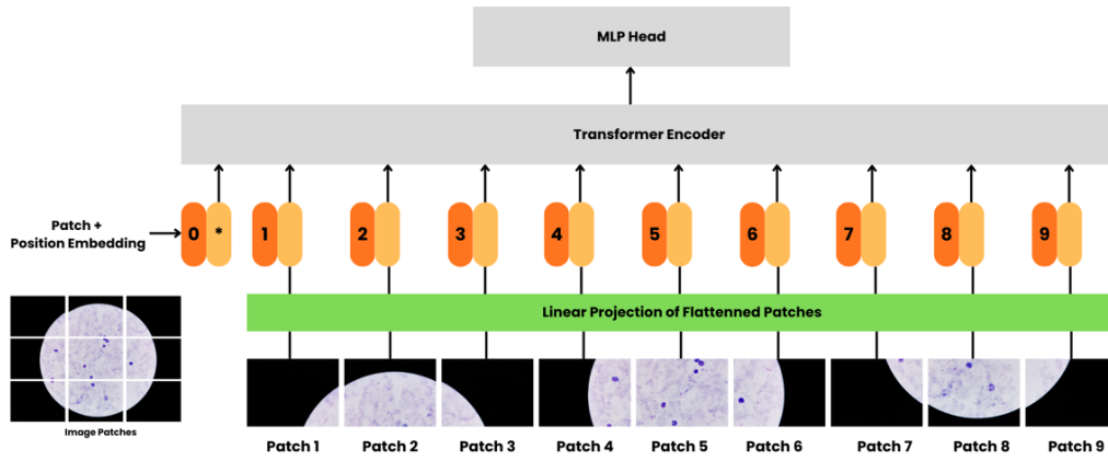
Figure 3. ViT Architecture
