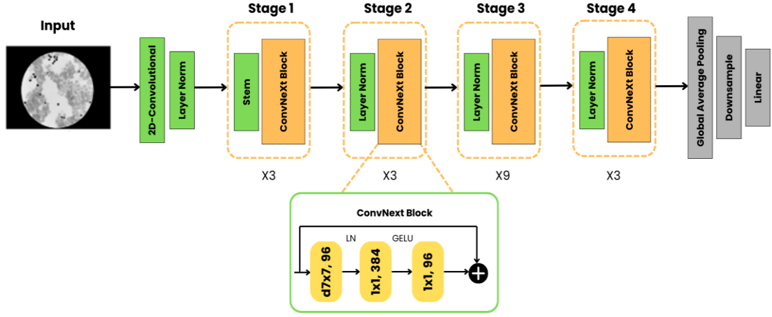
Figure 5. ConvNeXt Architecture
