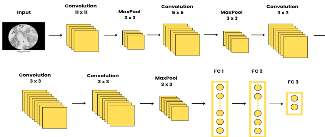
Figure 2. AlexNet Architecture
