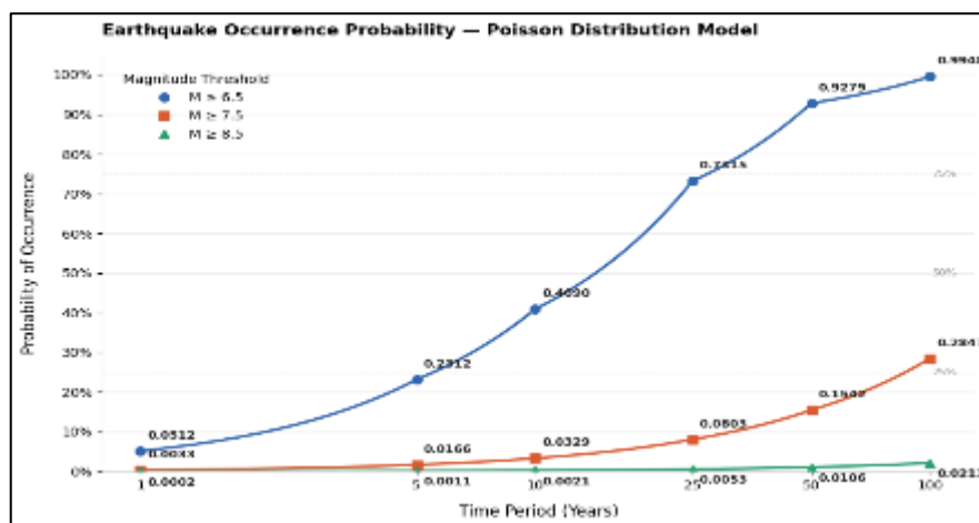
Figure 3. Earthquake probability trends for different magnitude thresholds (1–100 years)
