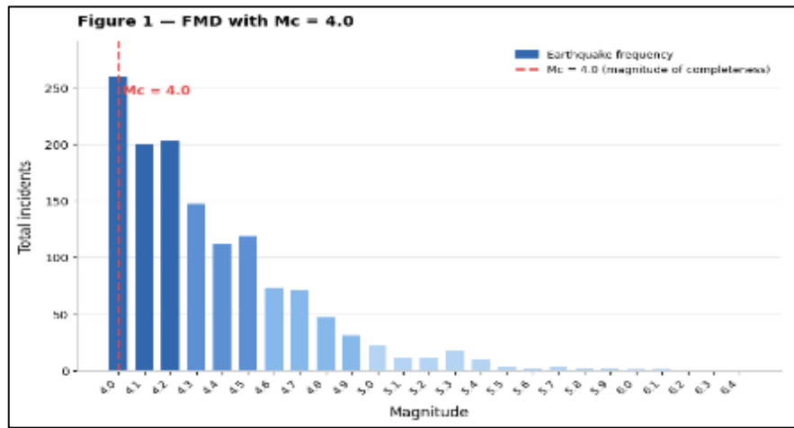
Figure 1. Frequency-Magnitude Distribution (FMD) with a magnitude of M_c = 4.0
