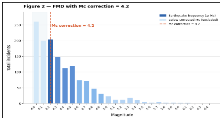
Figure 2. Frequency-Magnitude Distribution (FMD) with M_{c(\text{correction})} = 4.2
